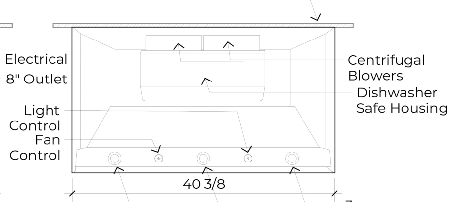
BOTTOM VIEW
